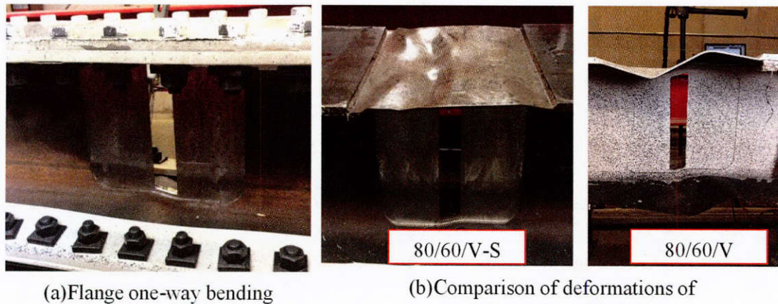
Figure 8.60: Observed failure on Pile 80/60/V-S and Pile 80/60/V
