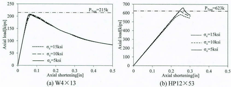
Figure 6.6: Effects of residual stresses on axial capacity
