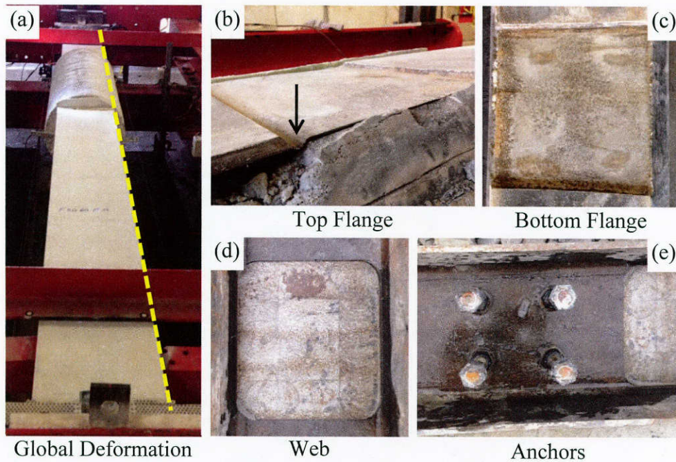
Figure 8.35: Pile 80/60(2)-F2/RA after testing
