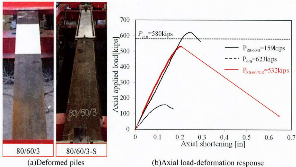
Figure 8.62: Comparison of Pile 80/60/3 and Pile 80/60/3-S
