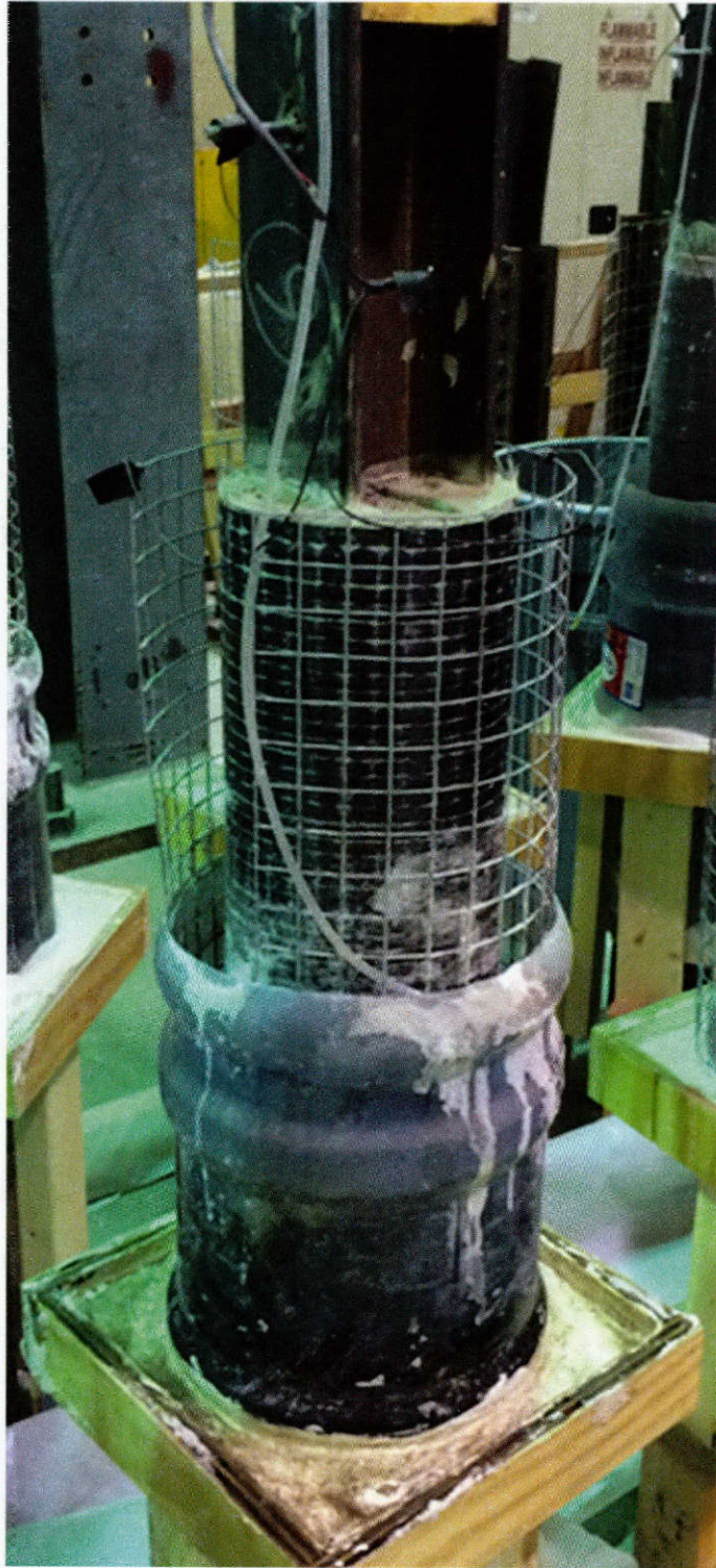
Figure 10.43: A damaged pile repaired with Repair System 2 (S2-12-Cor) showing no evidence of corrosion
