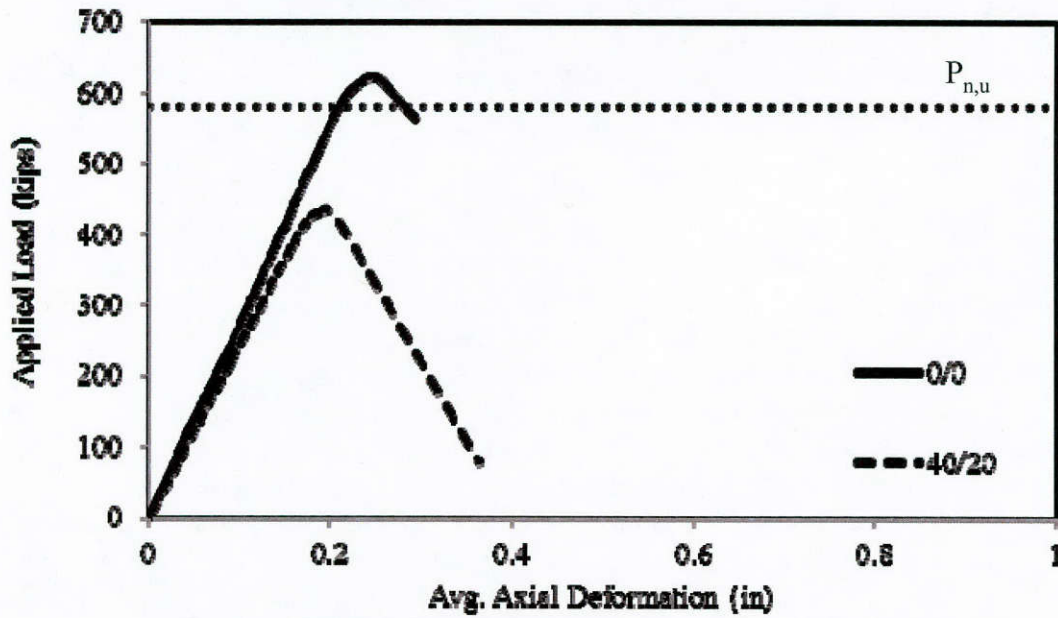
Figure 4.11: Axial load-shortening response of pile 40/20
