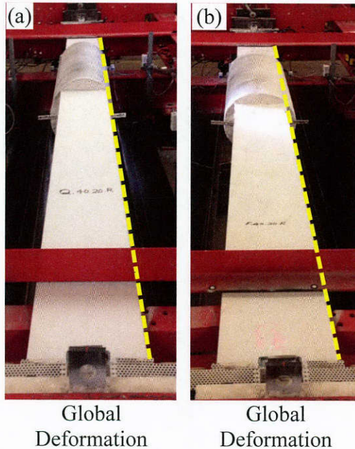
Figure 8.22: Piles 40/20 repaired with the F1 and F2 repair systems after testing
