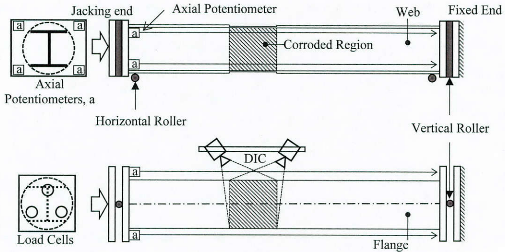
(a) Schematic Drawing of the Test Setup
