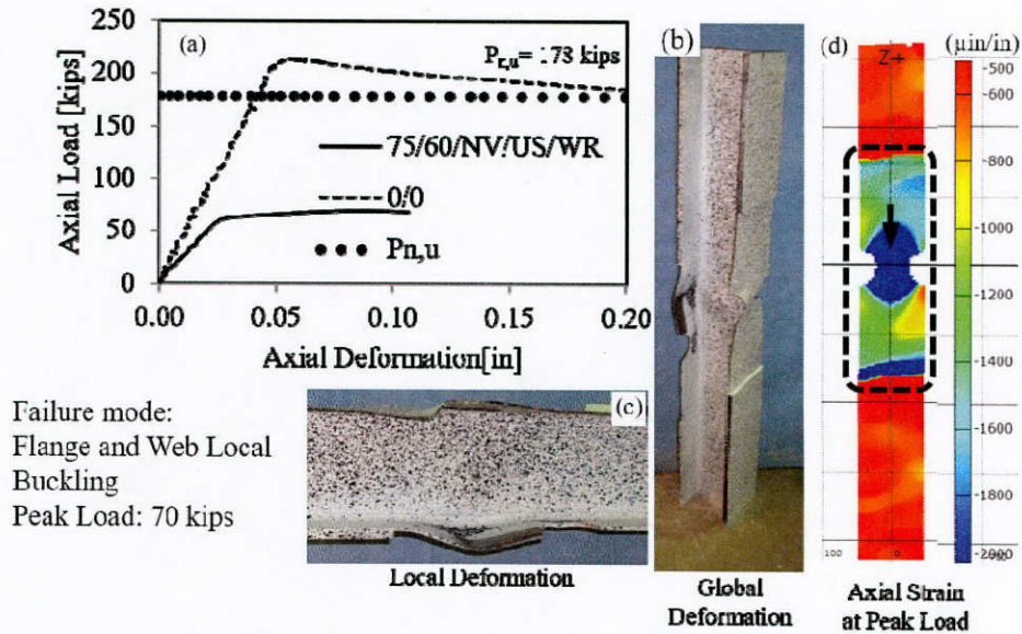
Figure 3.14: Failure mode and load-deformation response of pile 75/60/NV/US/WR
