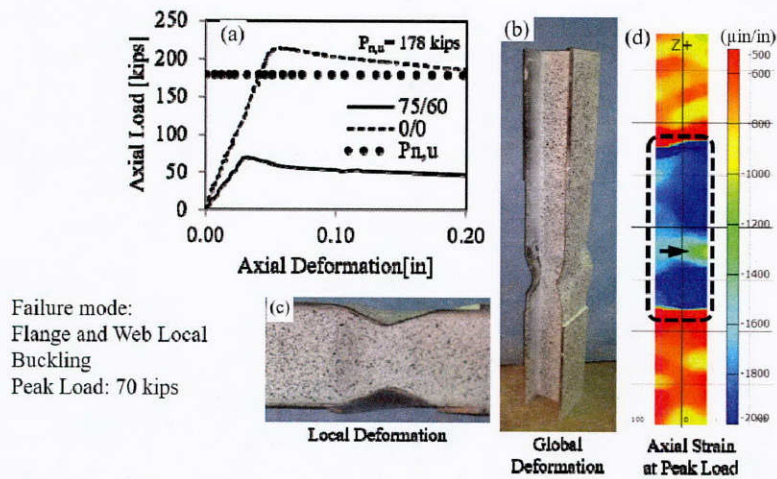
Figure 3.12: Failure mode and load-deformation response of pile 75/60
