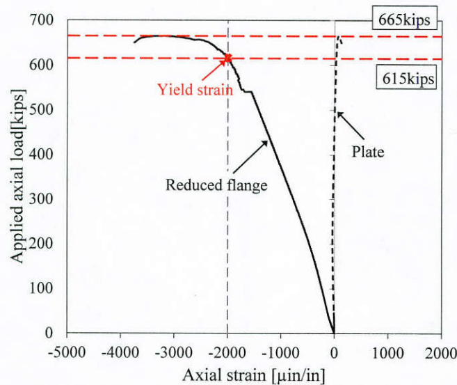
Figure 8.50: Axial strains of the plate and the reduced flange of Pile 40/20-S
