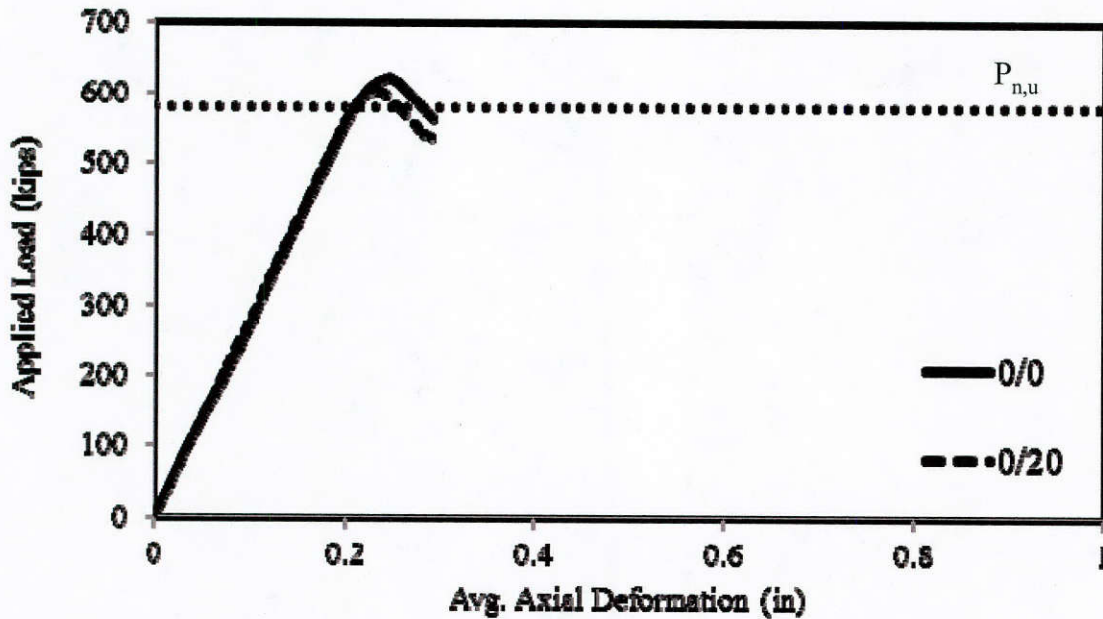
Figure 4.9: Axial load-shortening response of pile 0/20
