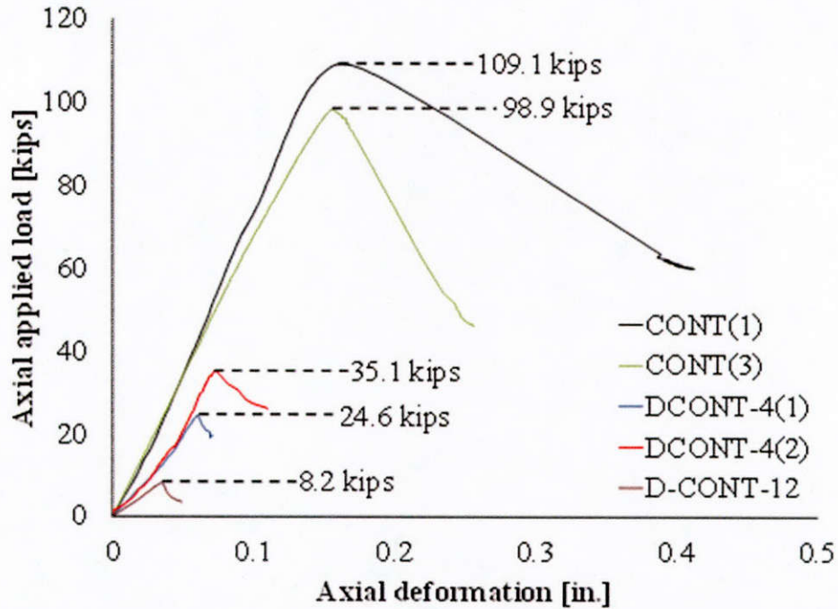
Figure 10.36: Axial load vs. axial deformation curves of the damaged control piles (DCONT-4 and DCONT-12)
