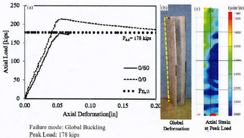
Figure 3.8: Failure mode and load-deformation response of pile 0/60
