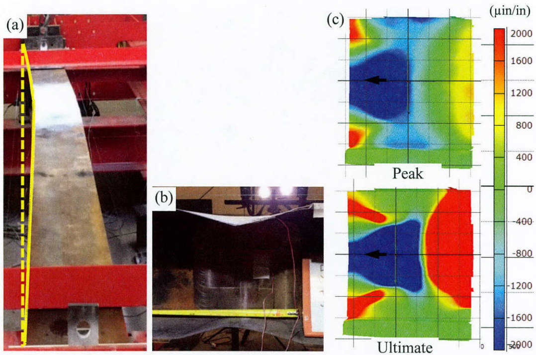
Figure 4.18: Global deformation, local deformation, and strain contours of pile 80/60
