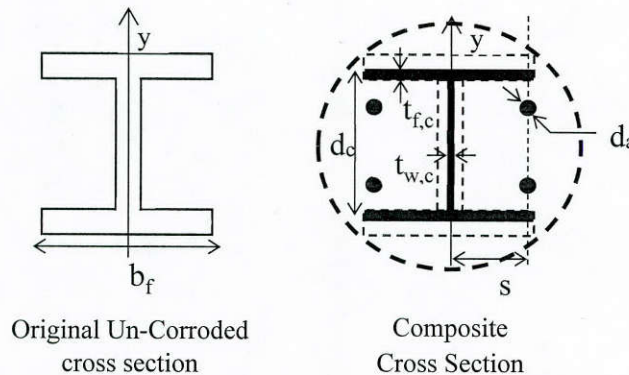
Figure 7.6. Configuration of the longitudinal reinforcing bars in the repaired pile
