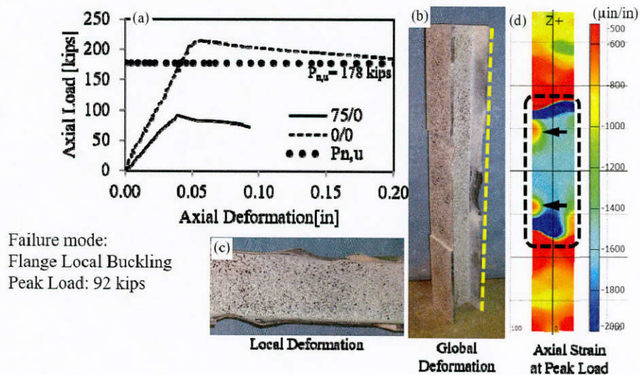
Figure 3.11: Failure mode and load-deformation response of pile 75/0
