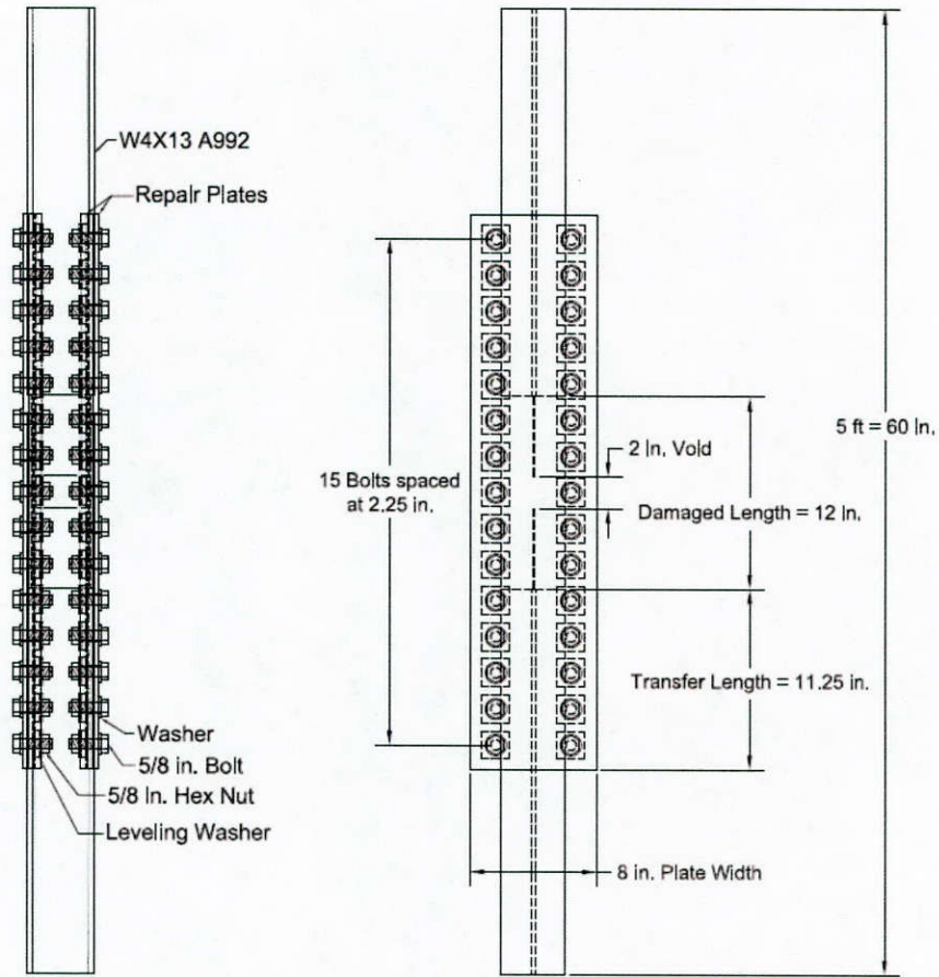
Figure 10.8: Design of Repair System 3 for the major repair
