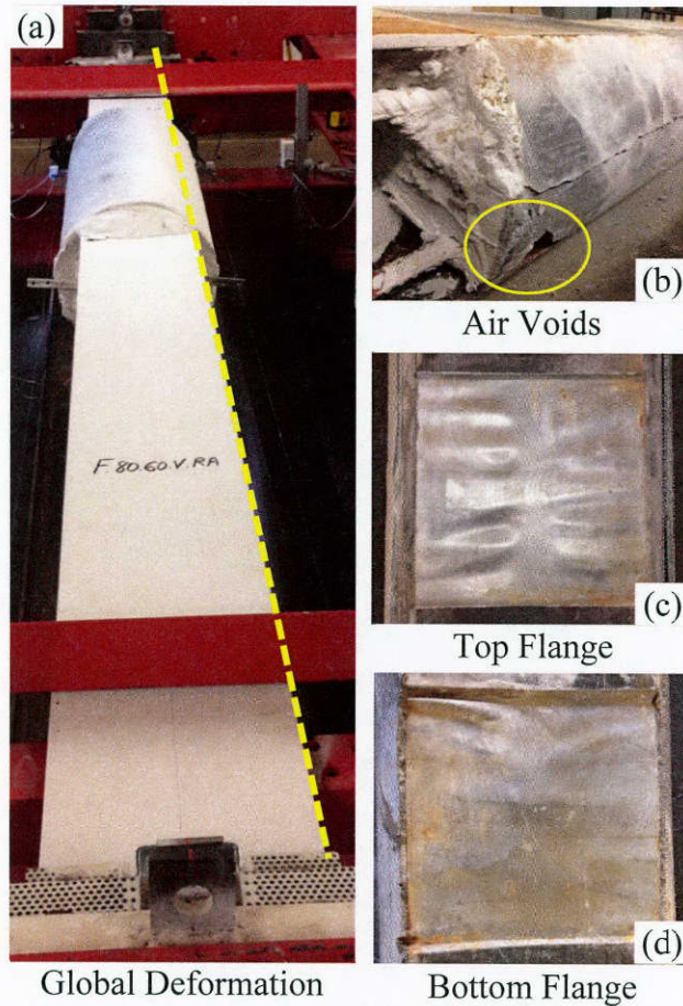
Figure 8.40: Pile 80/60/V-F2/RA after testing
