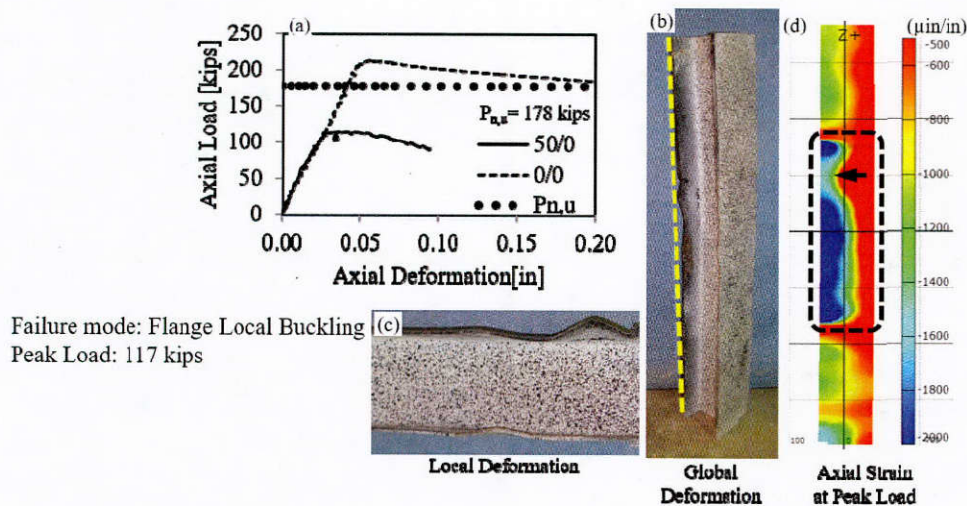
Figure 3.9: Failure mode and load-deformation response of pile 50/0
