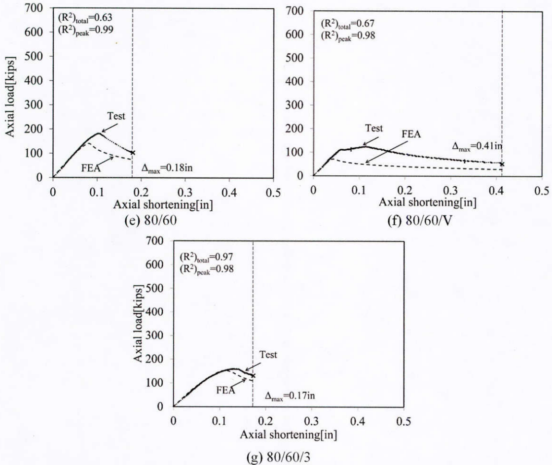
Figure 6.10: Comparison of axial load-deformation responses from test and FEA of HP12×53
