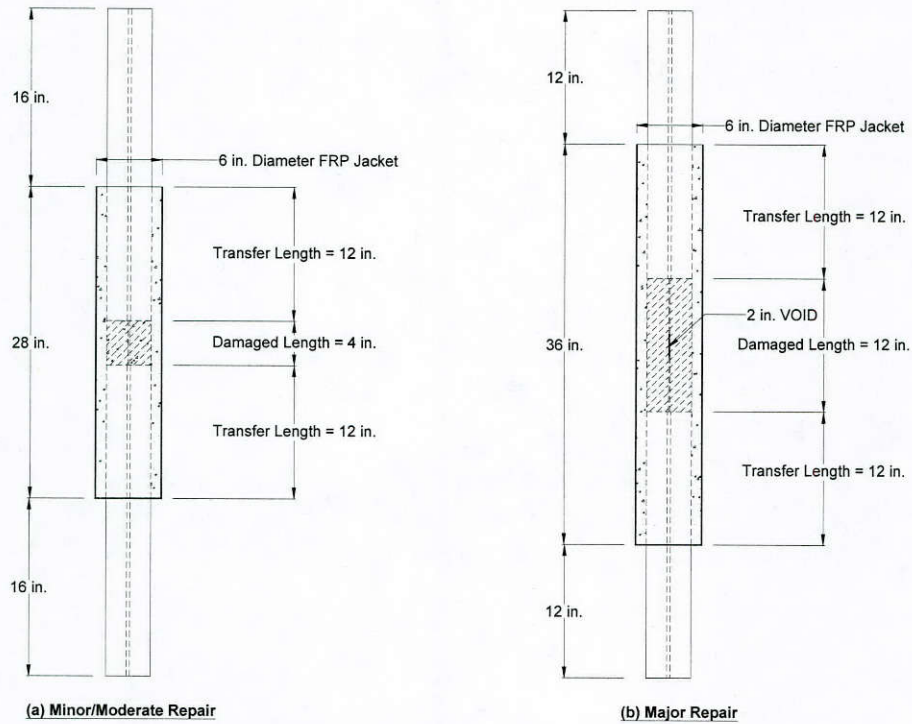
Figure 10.4: Length of the FRP jackets used for the minor repair case and the minor repair case
