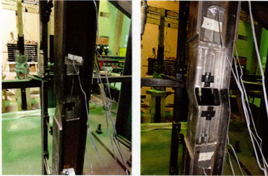
Figure 10.26: Failure of 4-in. damaged control piles (DCONT-4) and 12-in. damaged control piles (DCONT-12)
