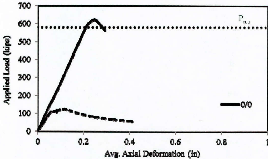
Figure 4.20: Axial load-shortening response of pile 80/60/V
