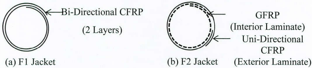
Figure 7.3: F1 and F2 jacket configurations
