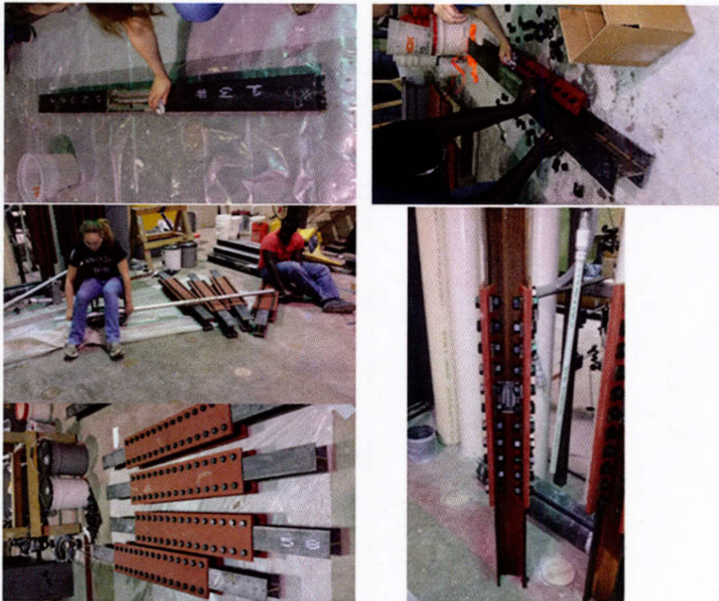
Figure 10.17: Fabrication of Repair System 3
