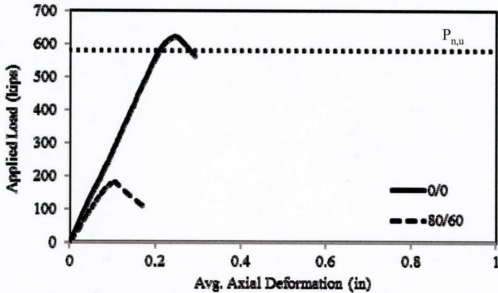
Figure 4.17: Axial load-shortening response of pile 80/60
