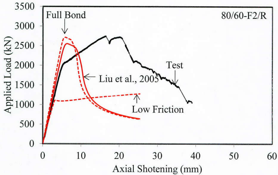
Figure 9.10: Comparison of full-bond, low friction, and Liu et al. bond-slip relationship
