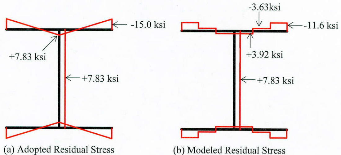
Figure 9.6: Residual stress magnitude and distribution
