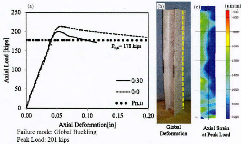
Figure 3.7: Failure mode and load-deformation response of pile 0/30
