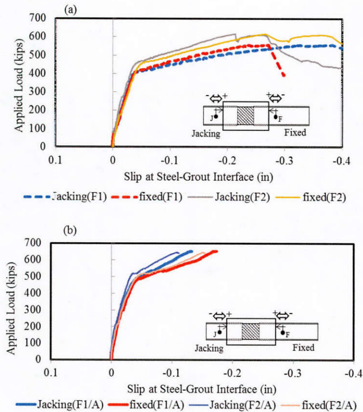
Figure 8.30: Comparing the slip at steel-grout interface of 80/60 repaired piles (a) piles without mechanical anchors, and (b) piles with mechanical anchors.
