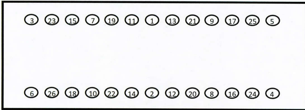
Figure 12.10: Bolt tightening sequence
