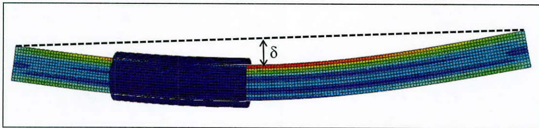
Figure 9.4: Applied initial global imperfection to FE models
