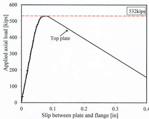
Figure 8.64: Slip of the steel repair plates of Pile 80/60/3-S
