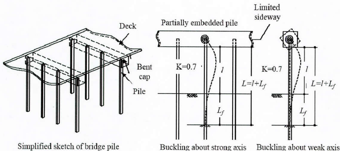
Figure 4.1: Schematic view of bridge piles and buckling modes
