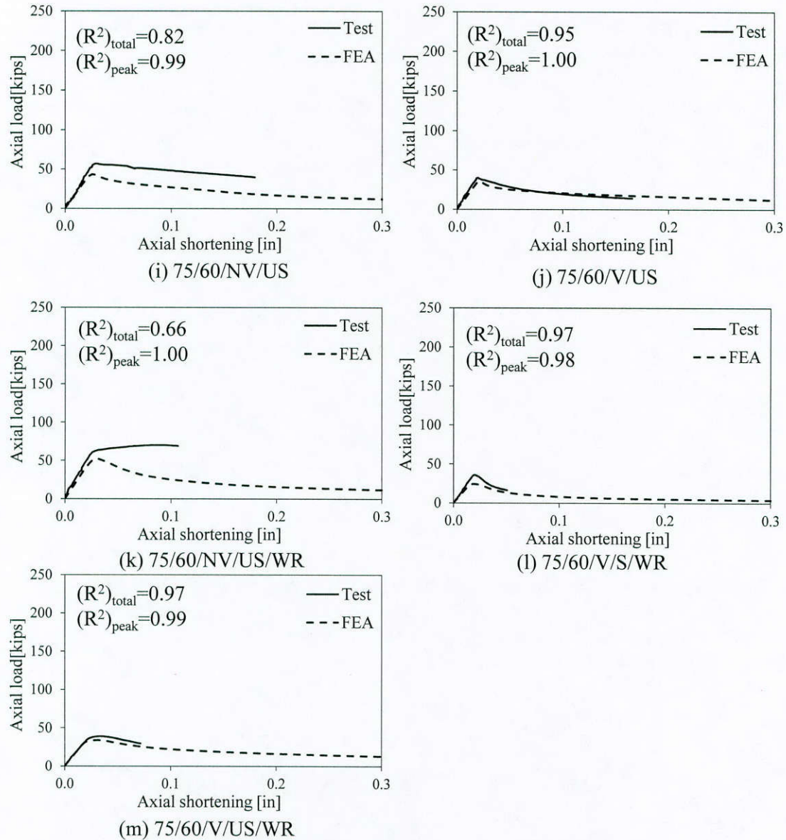
Figure 6.8: Comparison of axial load-shortening responses from tests and FEA of W4×13
