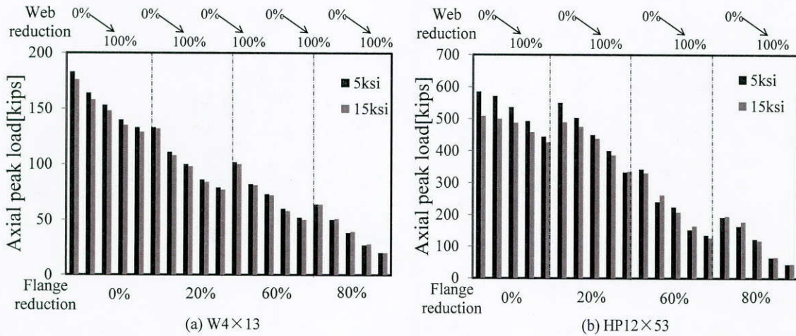
Figure 6.13: Axial peak loads of piles with different residual stresses
