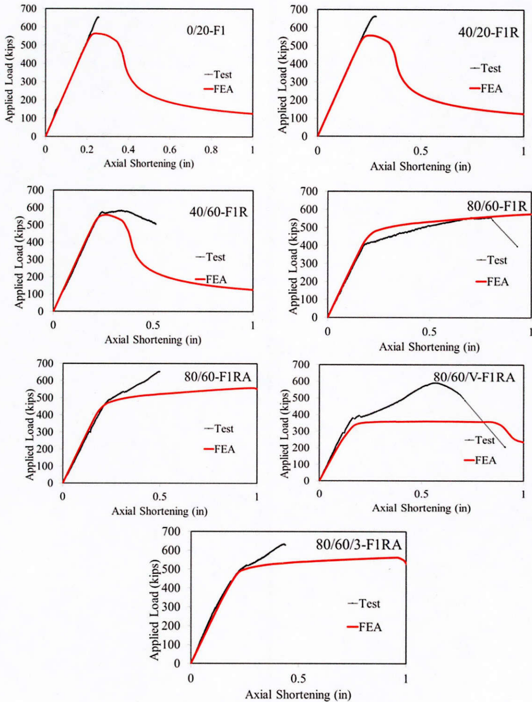
Figure 9.17: Comparison of the test and FE load-shortening response for the piles repaired with F1 jacket
