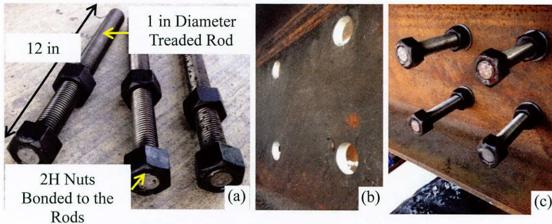
Figure 8.4: Installation of headed-stud anchor
