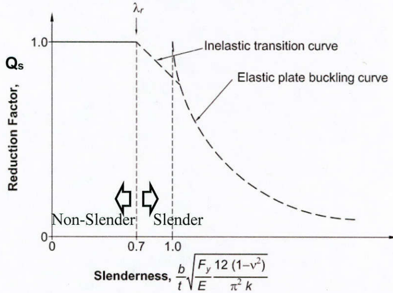
Figure 2.3: Slender un-stiffened element reduction factor (AISC, 2010)
