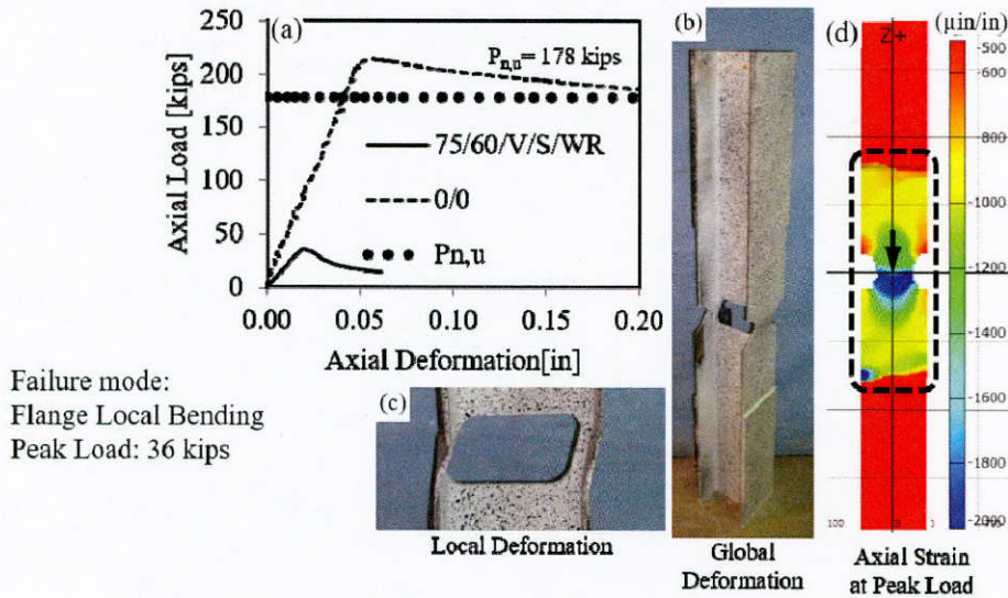
Figure 3.16: Failure mode and load-deformation response of pile 75/60/V/S/WR
