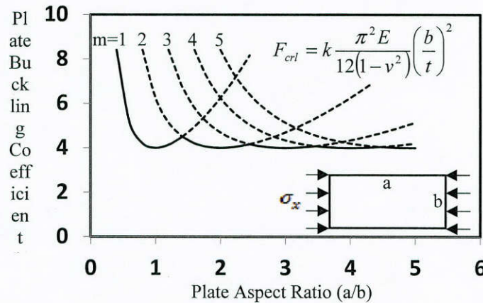
Figure 2.2: Correlation between Plate Buckling Coefficient and Aspect Ratio (adapted from Timoshenko, 1961)
