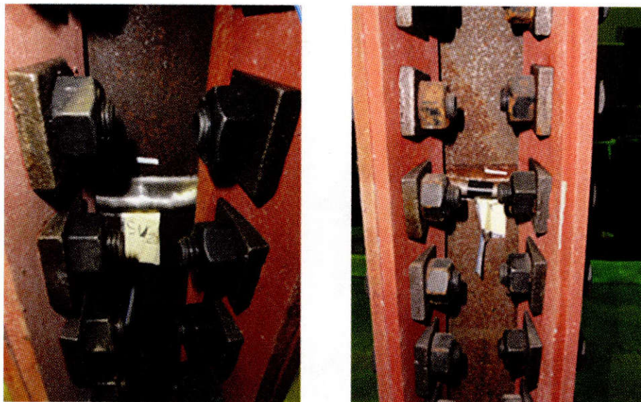
Figure 10.31: Crushing of 4-in. damaged region of the test piles repaired with Repair System 3
