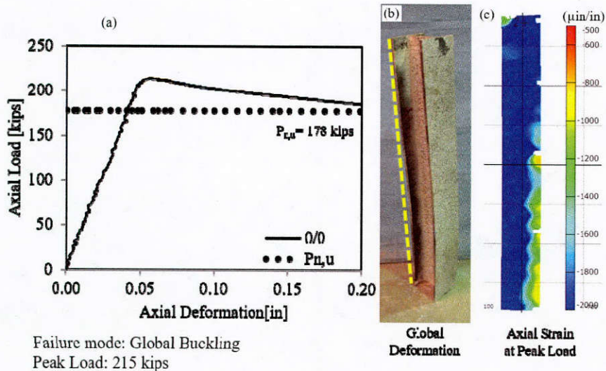
Figure 3.6: Failure mode and load-deformation response of pile 0/0
