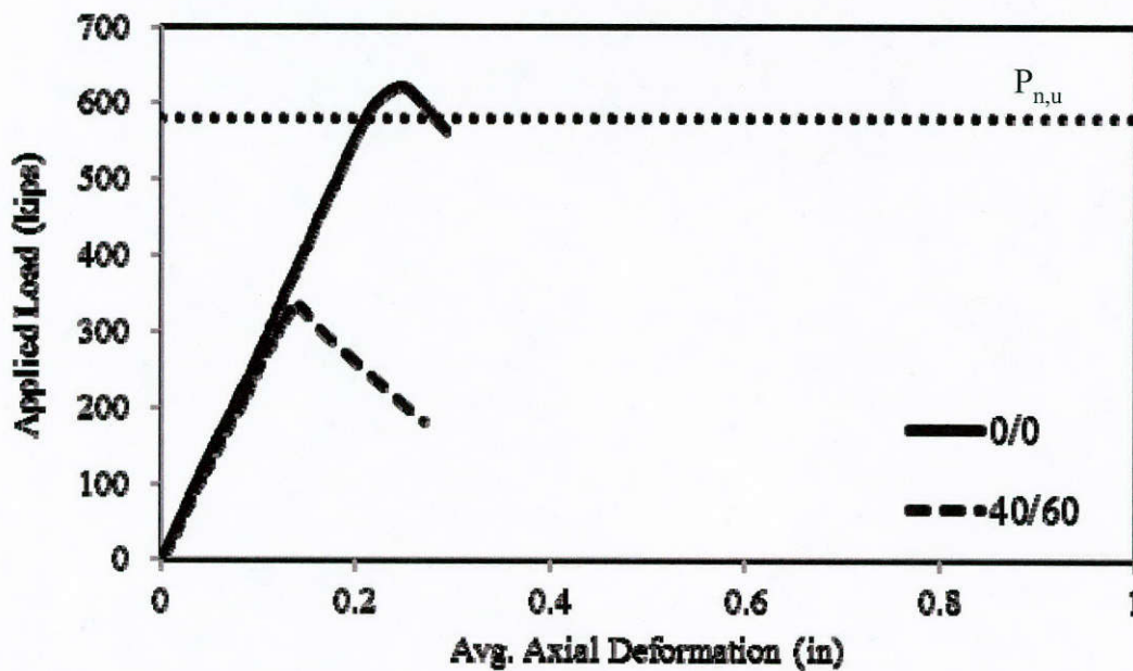
Figure 4.14: Axial load-shortening response of pile 40/60
