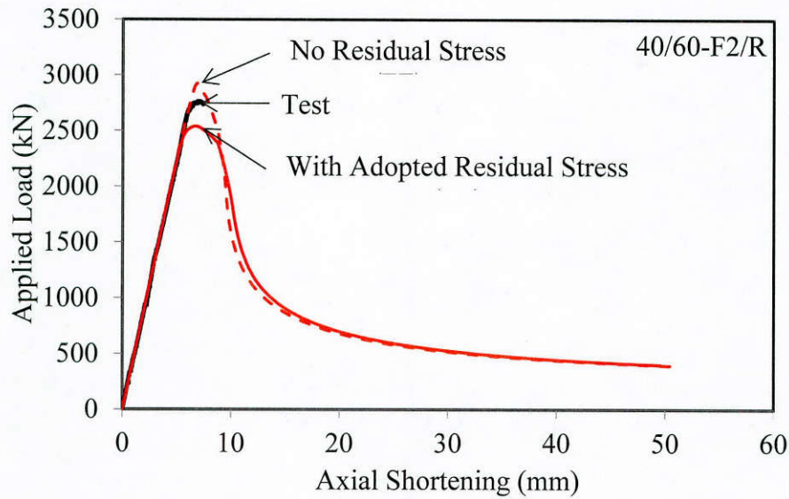
Figure 9.7: Effect of residual stress on axial load-shortening response
