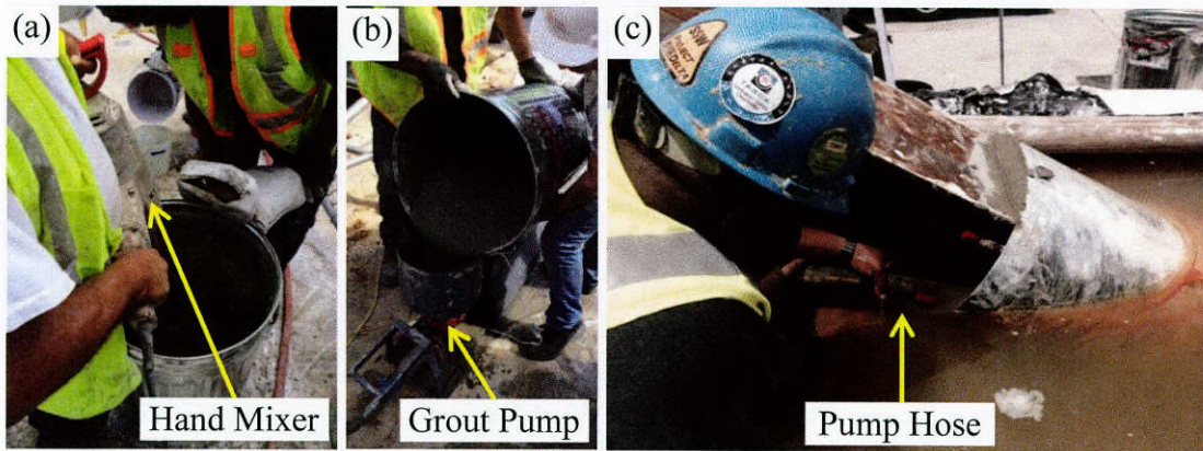
Figure 8.8: Grout casting
