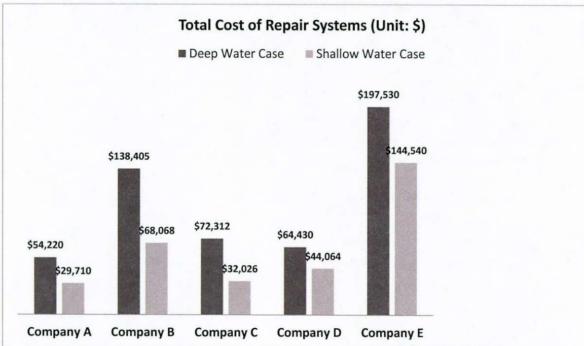
Figure 11.6: Total Cost of Repair Systems in Shallow and Deep Water Case
