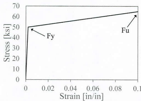
Figure 6.4: Stress-strain relationship of steel used in FEA
