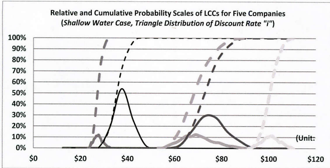
Figure 11.20: Probability Scales of LCCs for Five Companies under Probabilistic Interest Rates (Shallow Water, n=75)
