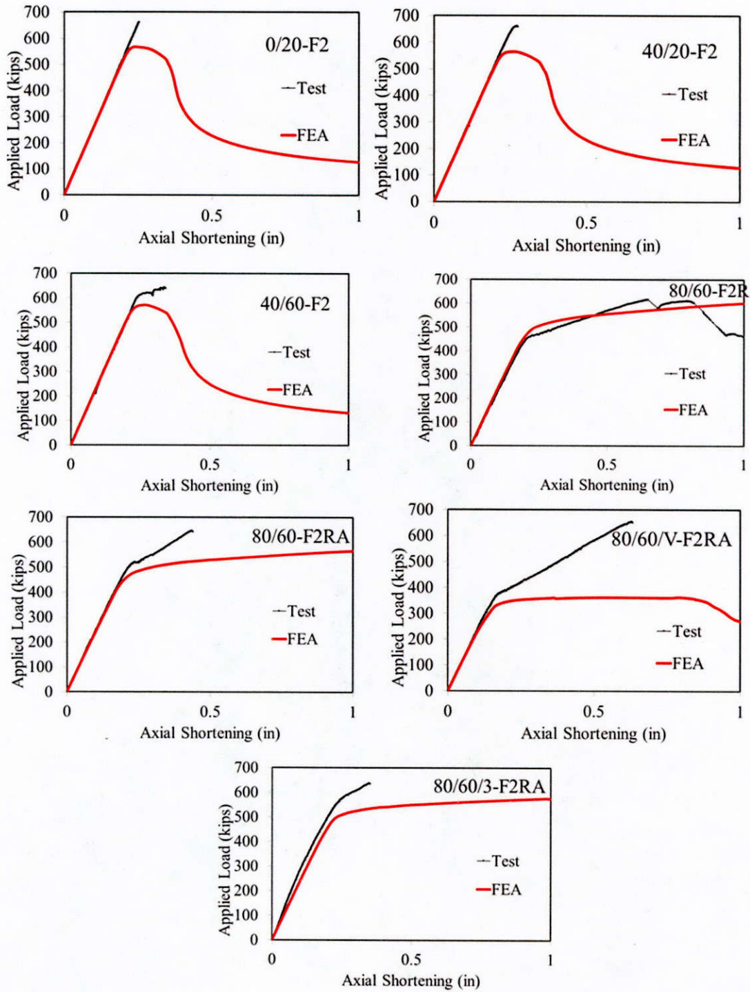
Figure 9.18: Comparison of the test and FE load-shortening response for the piles repaired with F2 jacket
