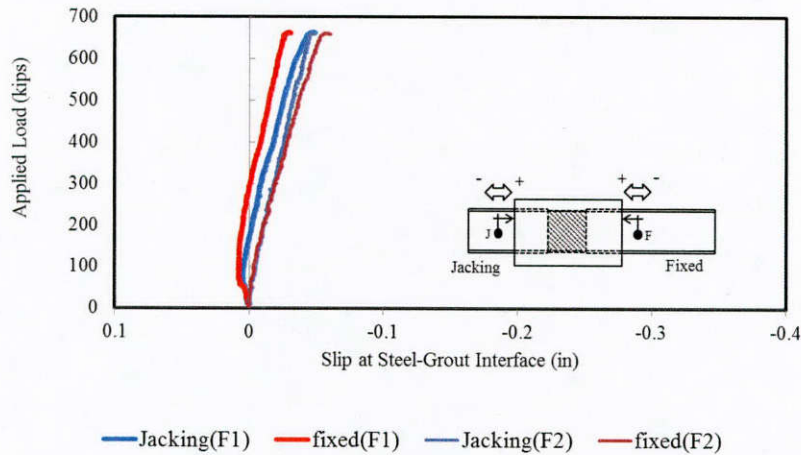
Figure 8.23: Comparing the slip at steel-grout interface of 40/20 repaired piles
