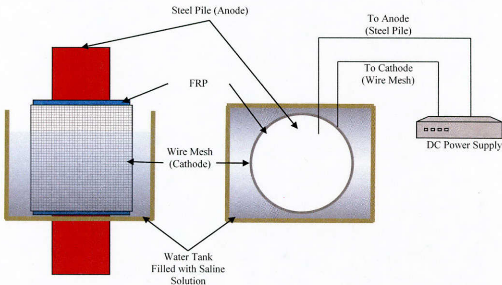
Figure 10.20: Schematic of accelerated corrosion process
