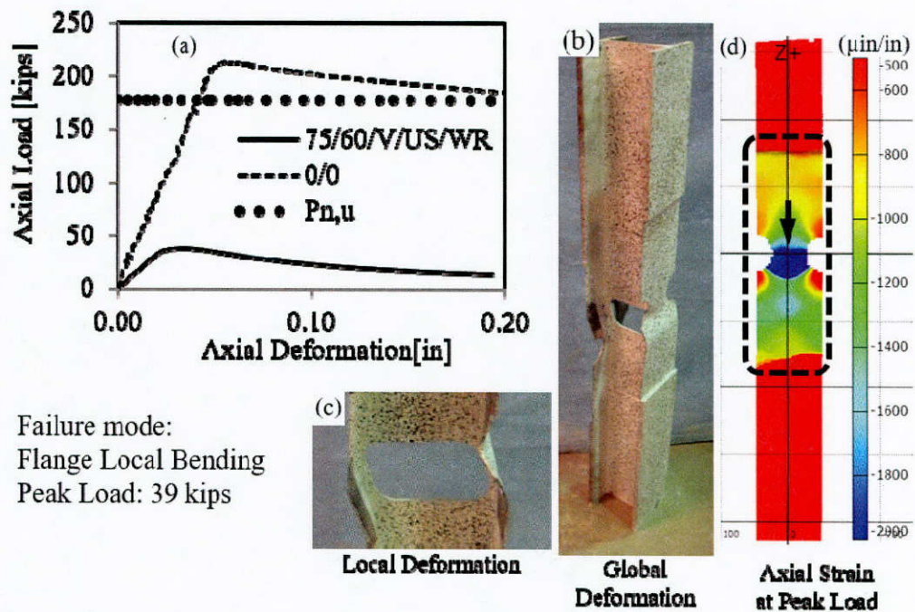
Figure 3.18: Failure mode and load-deformation response of pile 75/60/V/US/WR
