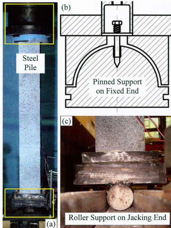
Figure 3.3. Test setup for small-scale piles
