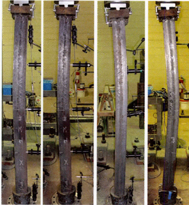
Figure 10.25: Failure of an undamaged control column (CONTs)
