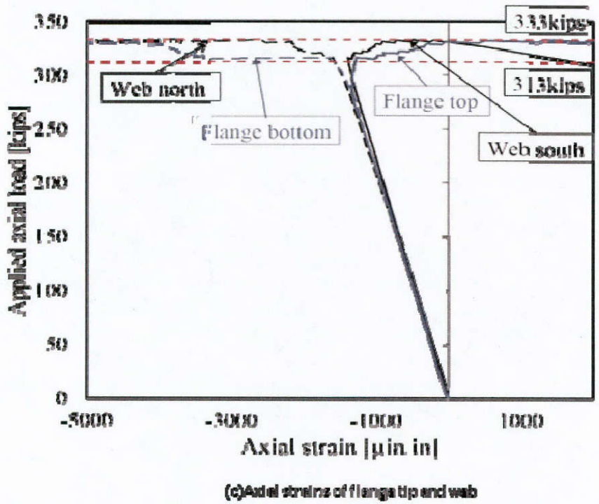
Figure 4.16: Flange and web local buckling of pile 40/60
