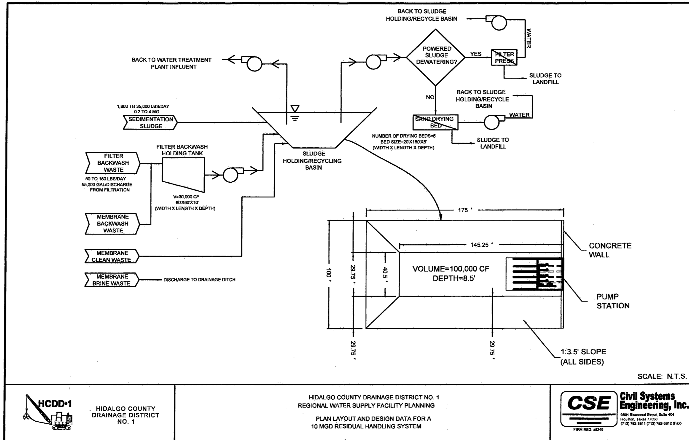
Figure 6-7. Residual Handling Process for a 10 MGD WTP
