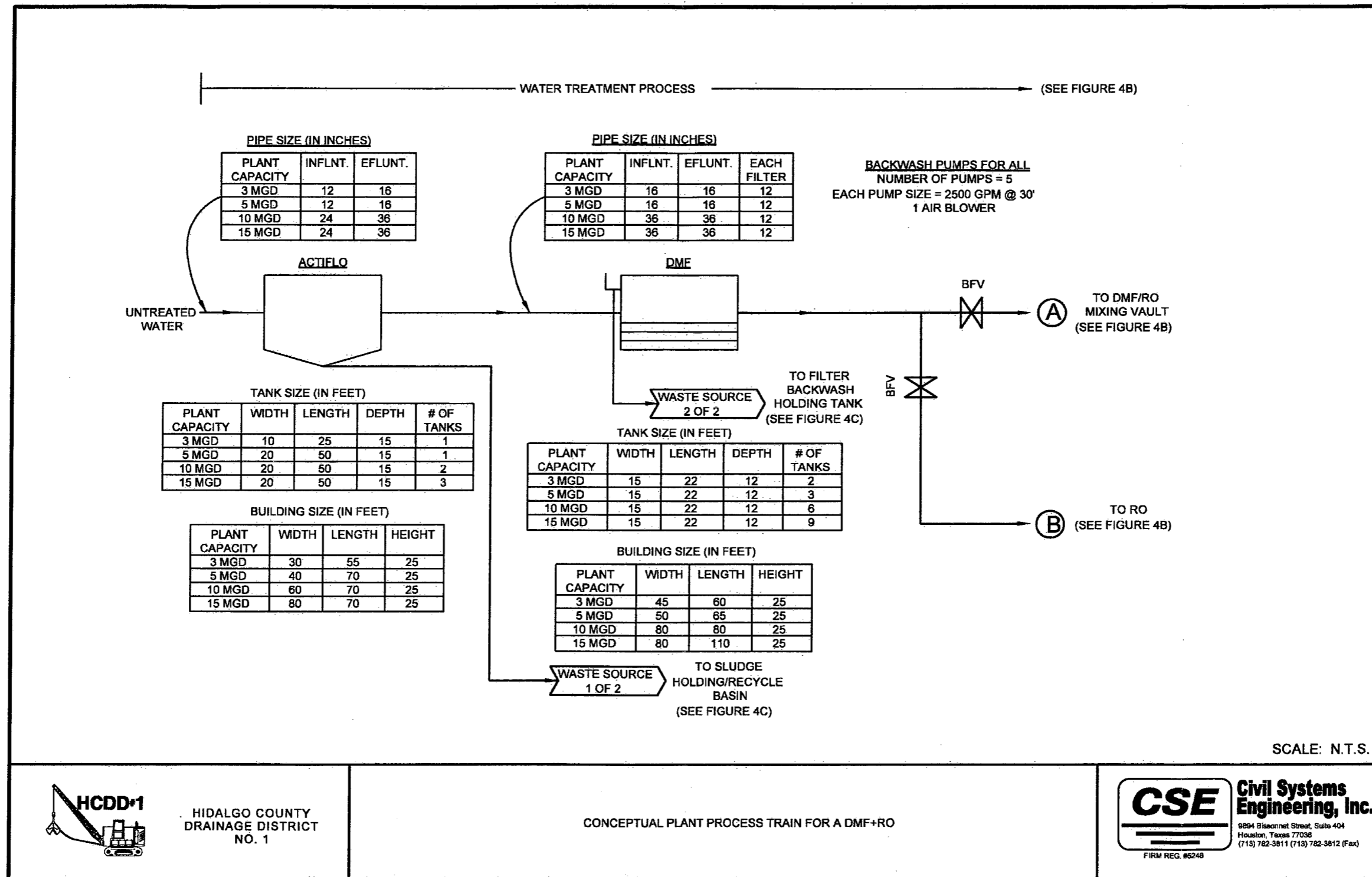
Figure 7-4-1 Conceptual WTP Process Train for Alternative D - ACTIFLO + DMF + RO
