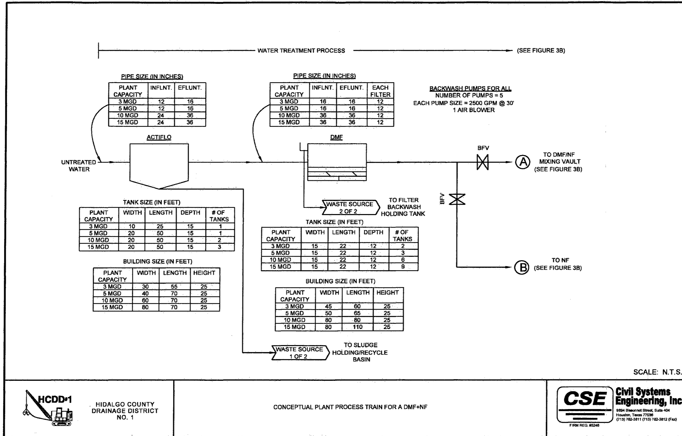
Figure 7-3-1. Conceptual WTP Process Train for Alternative C - ACTIFLO + DMF + NF
