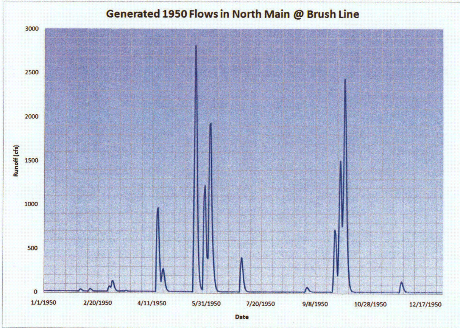
Figure 4-4. Synthetic Hydrograph (Combined Shallow Ground Water and Rainfall Runoff)
