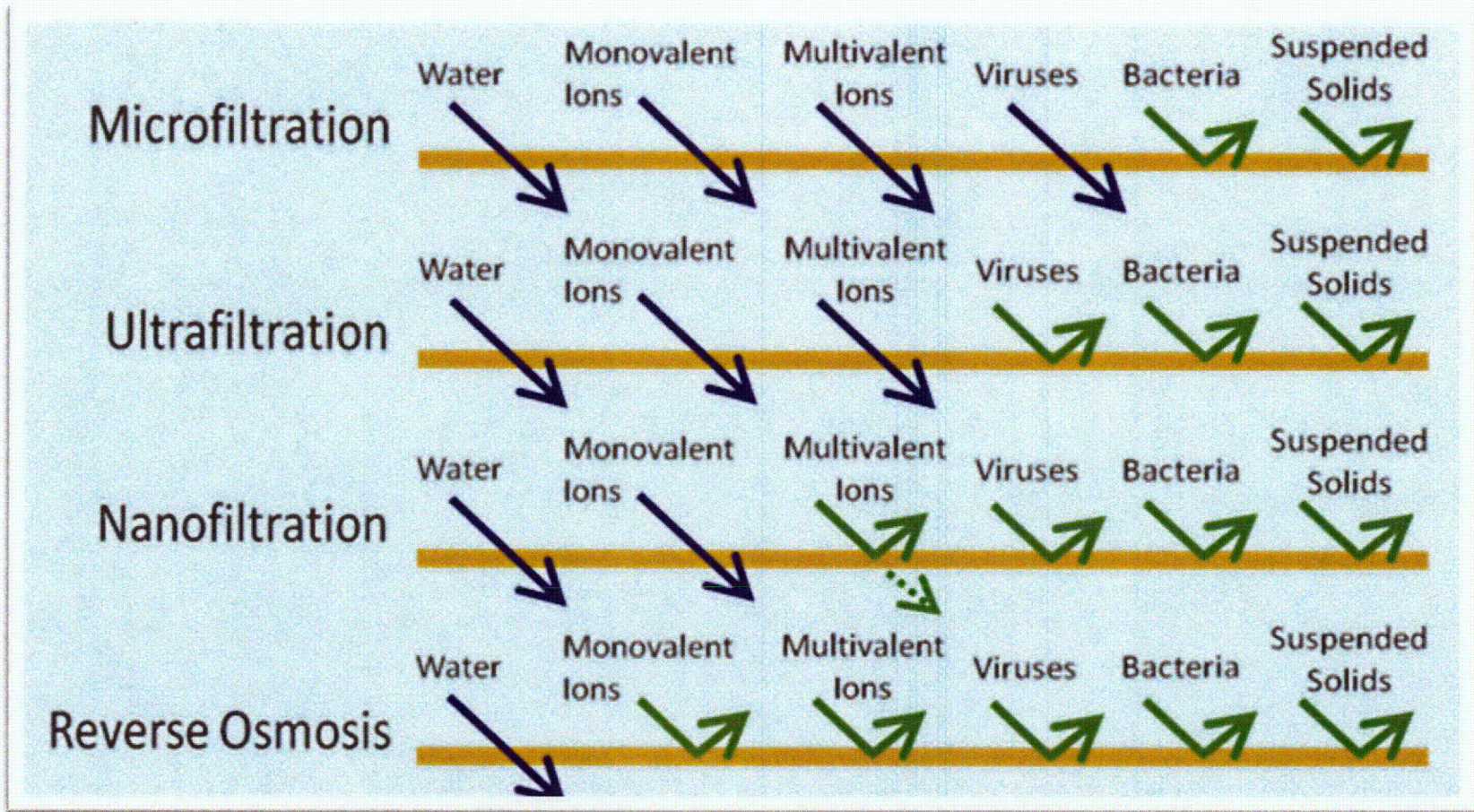
Figure 6-4. Effectiveness of Pressure-Driven Membrane Processes
