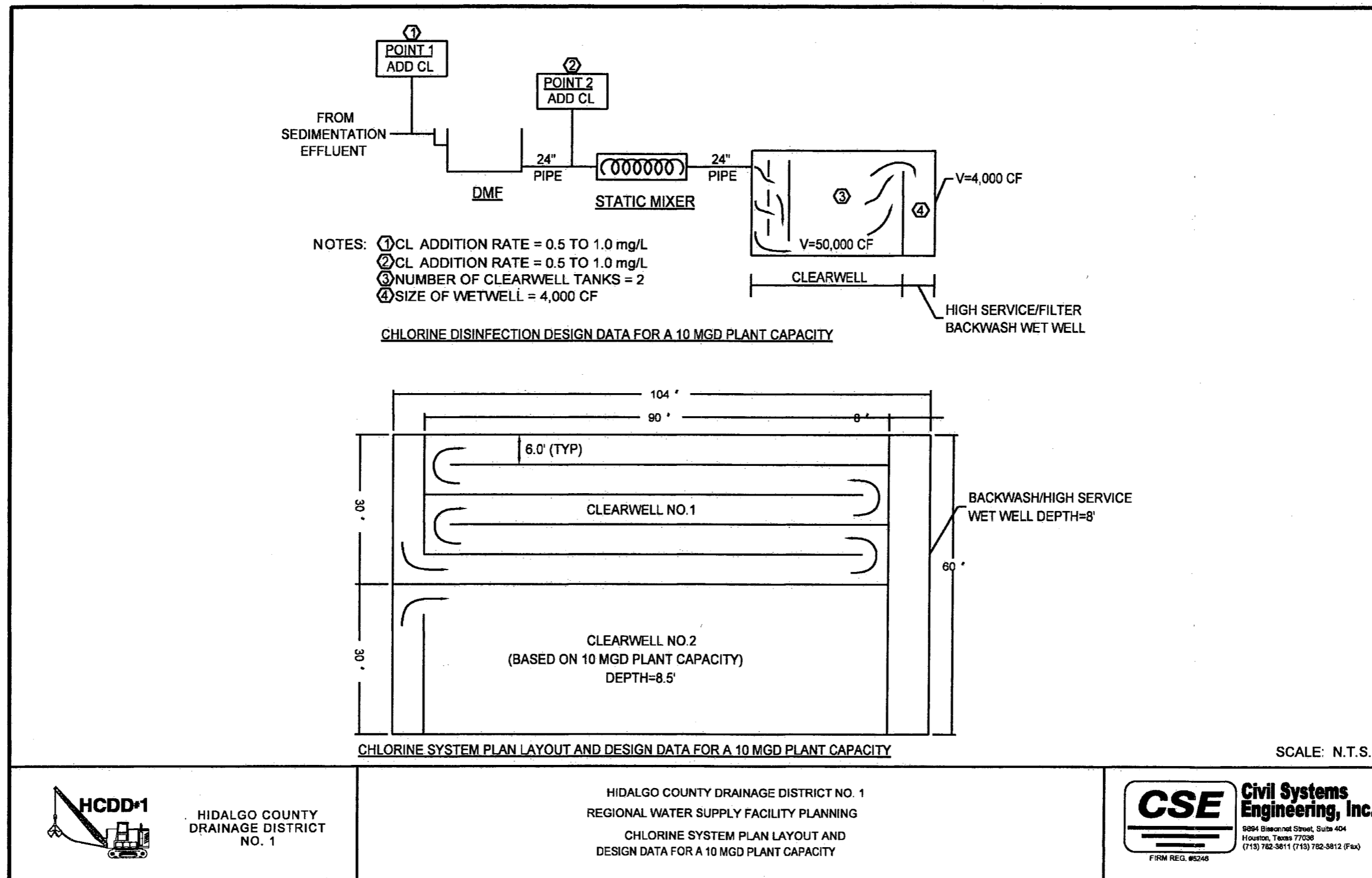
Figure 6-5. Chlorine System Layout
