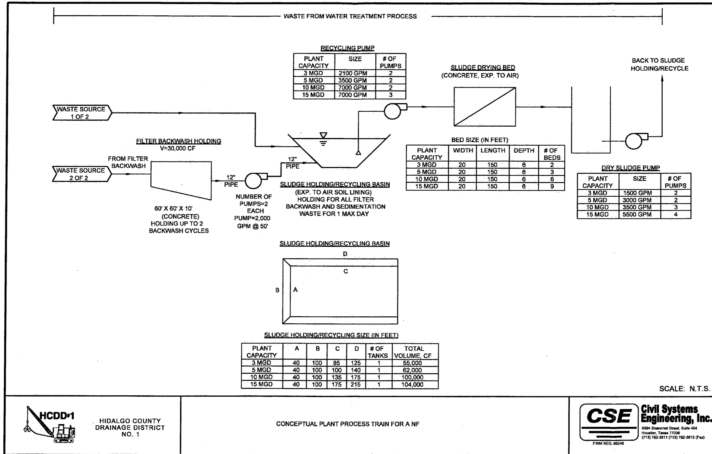
Figure 7-2-2 Conceptual WTP Process Train for Alternative B - ACTIFLO + NF
