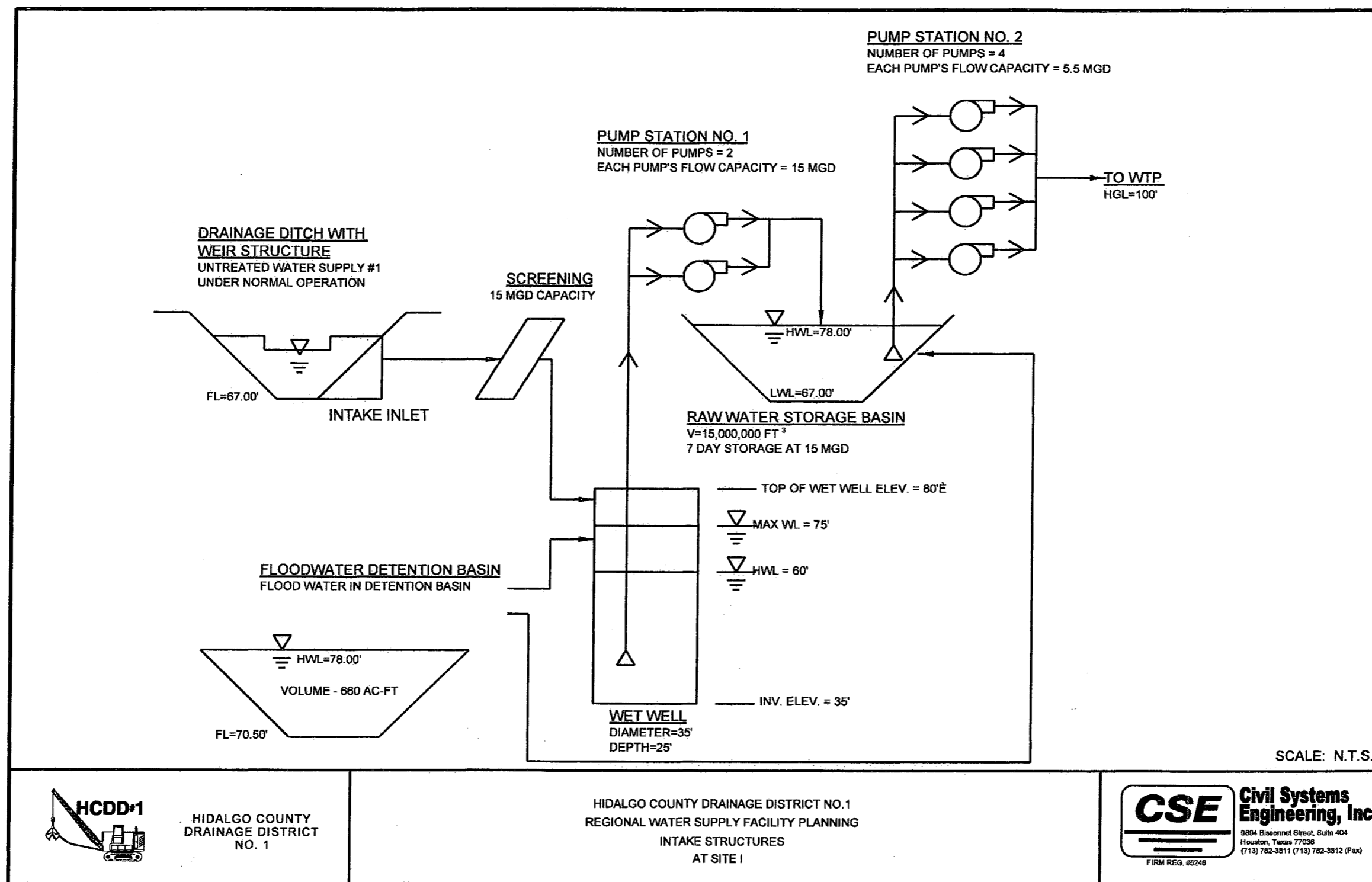
Figure 5-1. Intake Structures and Design Data at SITE I
