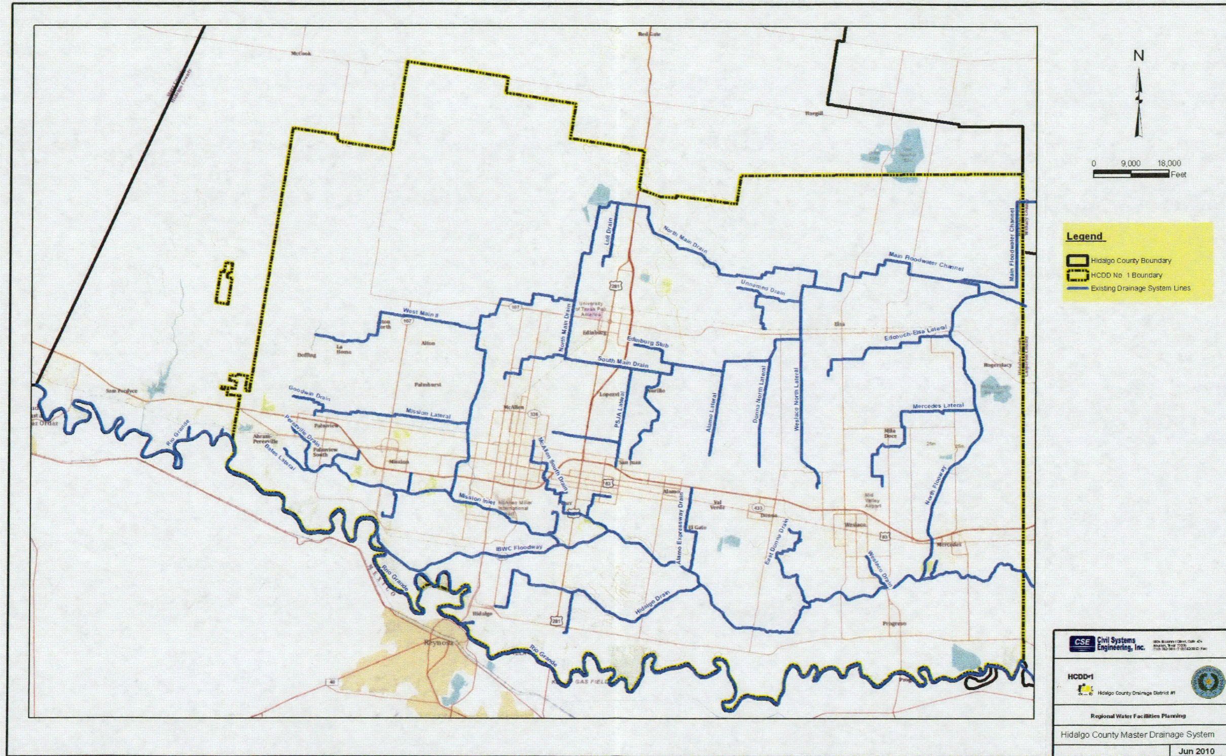
Figure 3-1. Hidalgo County Master Drainage Systems
