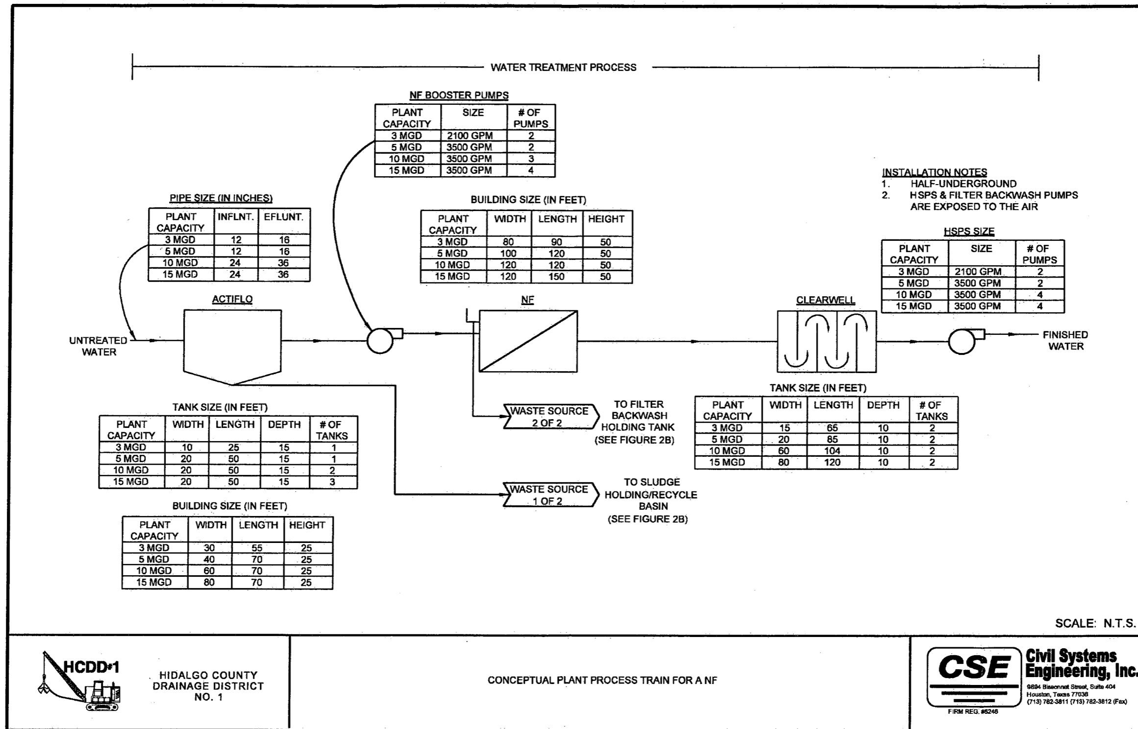
Figure 7-2-1 Conceptual WTP Process Train for Alternative B - ACTIFLO + NF
