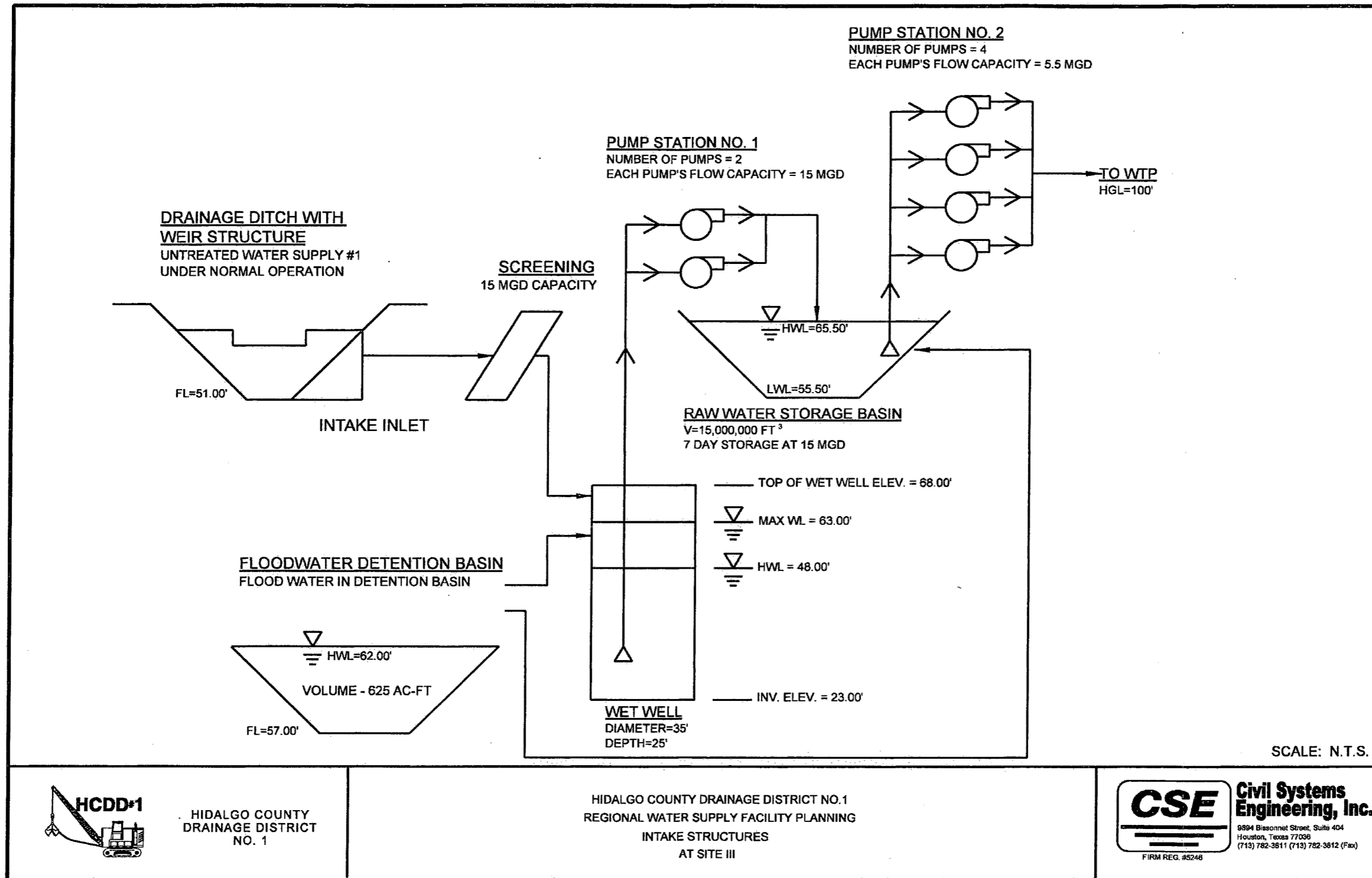
Figure 5-3. Intake Structures and Design Data at SITE III
