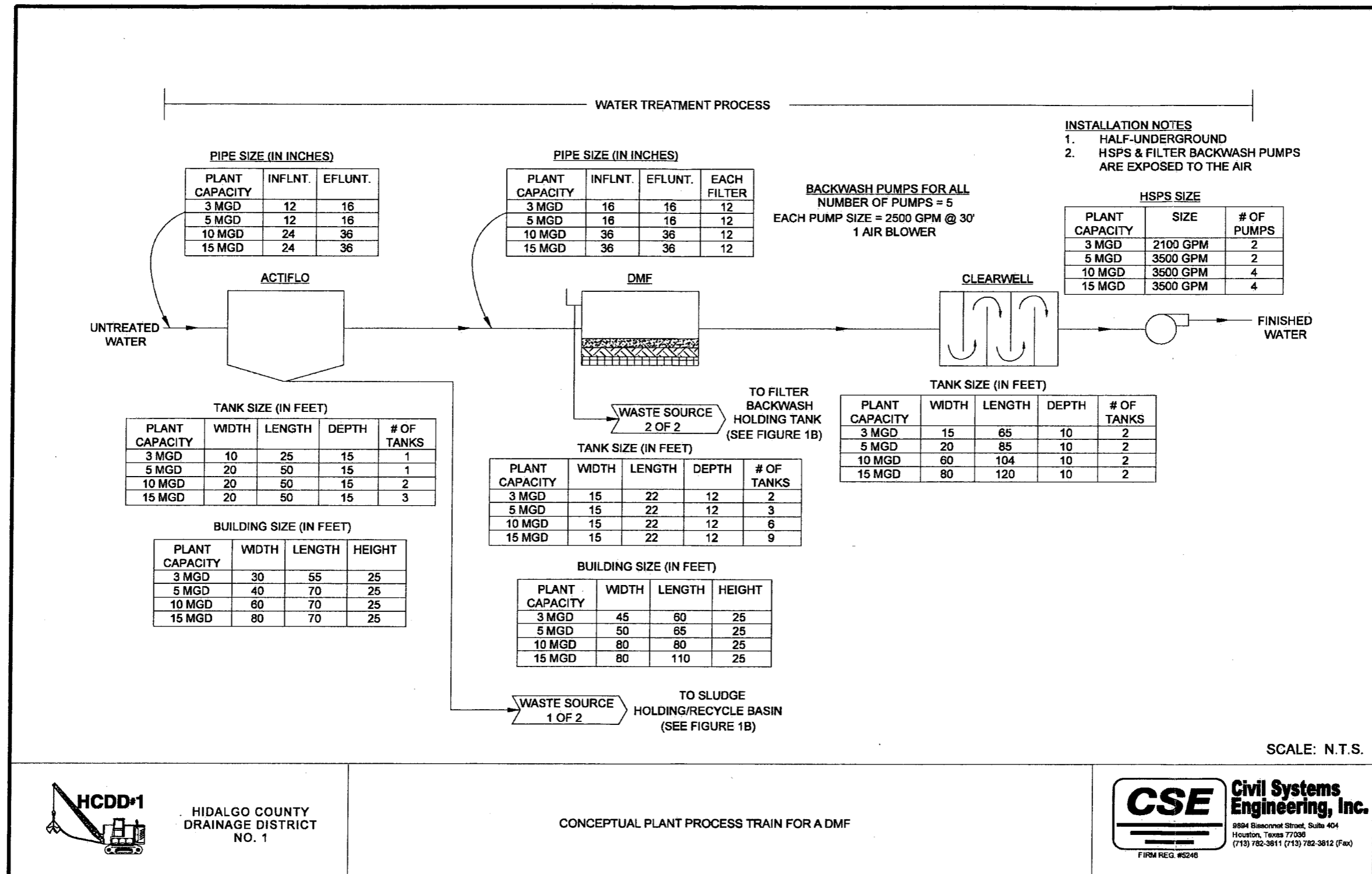
Figure 7-1-1 Conceptual WTP Process Train for Alternative A - ACTIFLO + DMF
