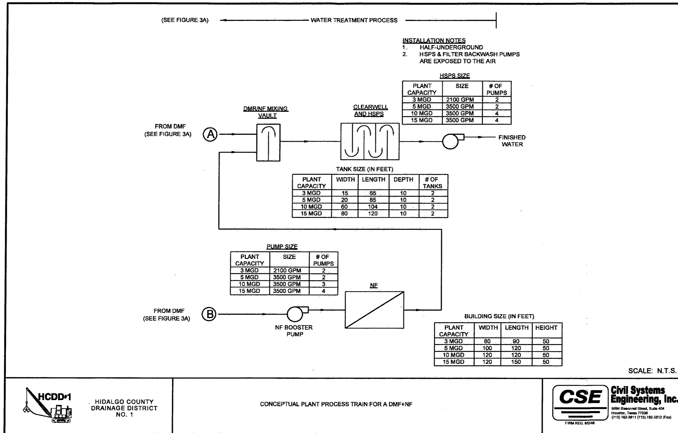
Figure 7-3-2. Conceptual WTP Process Train for Alternative C - ACTIFLO + DMF + NF
