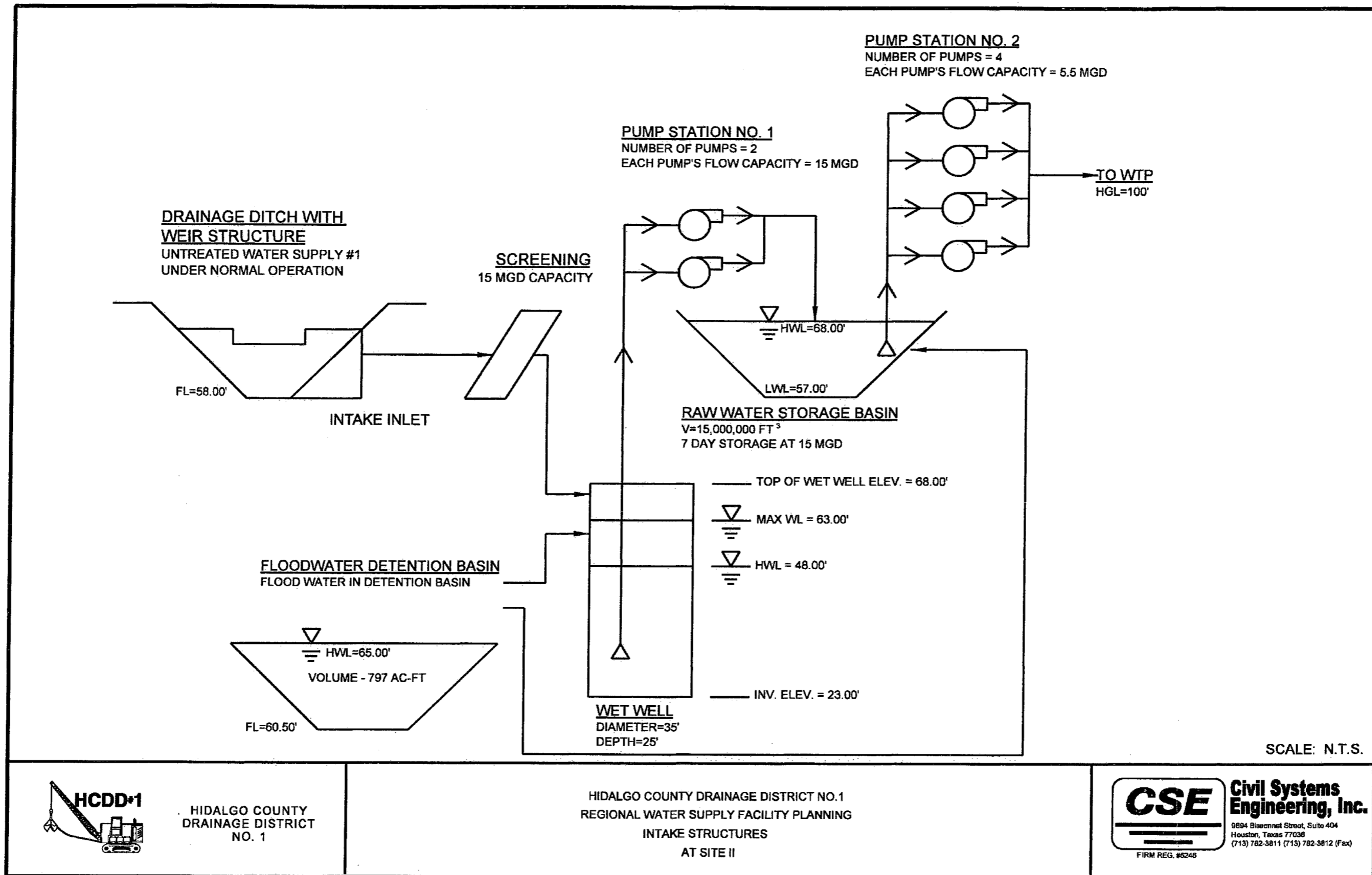
Figure 5-2. Intake Structures and Design Data at SITE II
