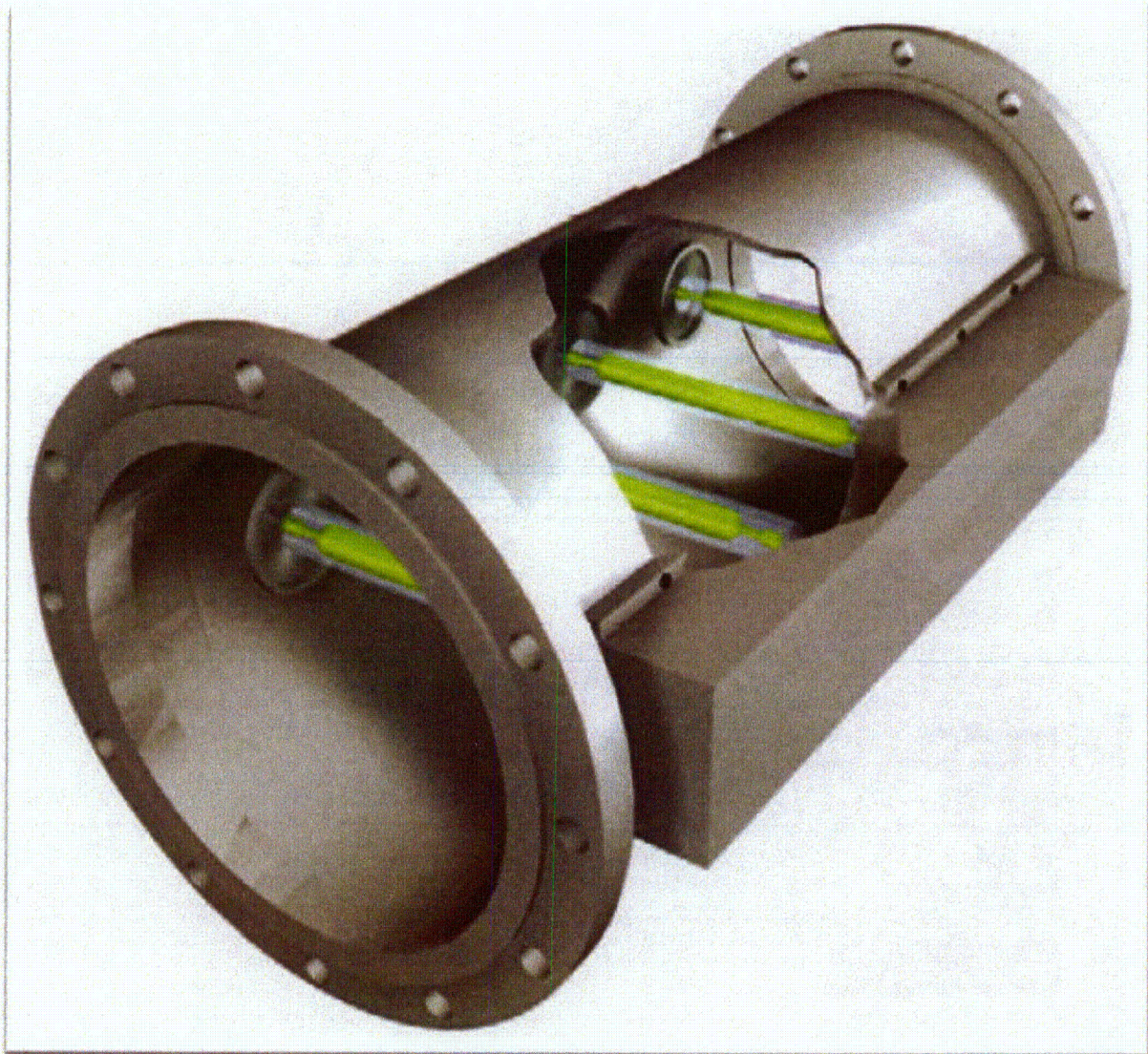
Figure 6-6. UV Disinfection Unit
