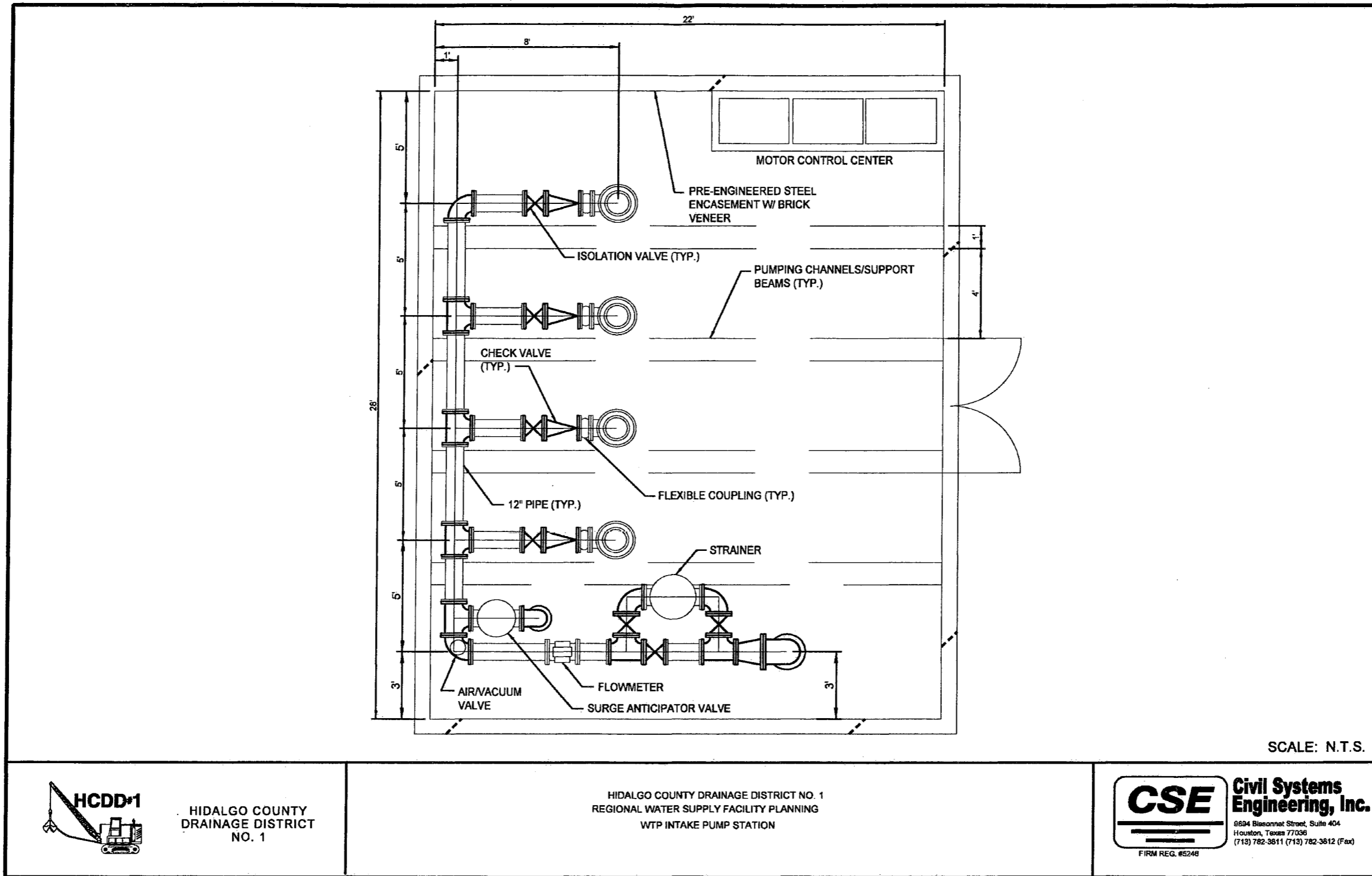
Figure 5-5. Pump Station II
