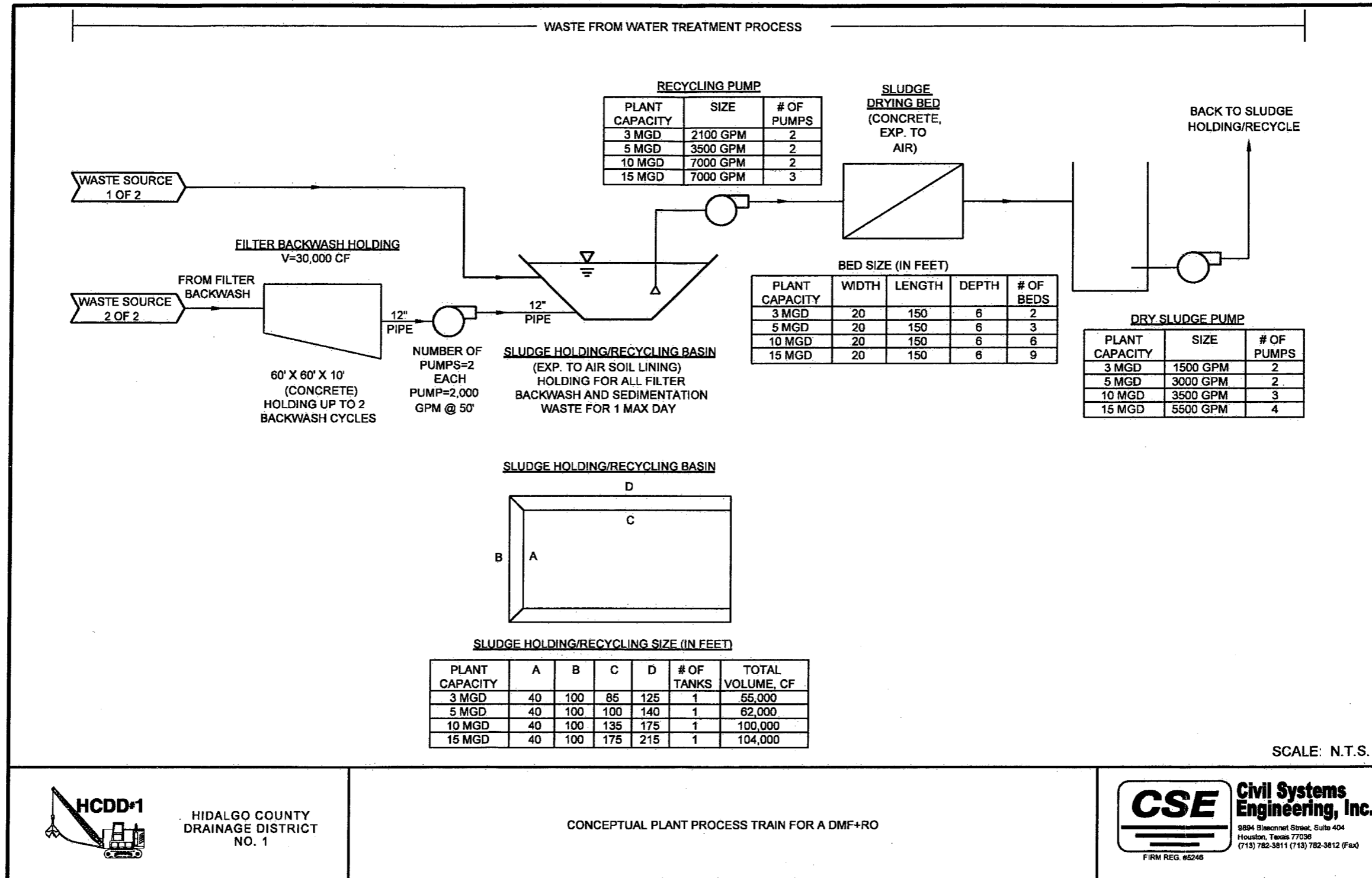
Figure 7-4-3. Conceptual WTP Process Train for Alternative D - ACTIFLO + DMF + RO
