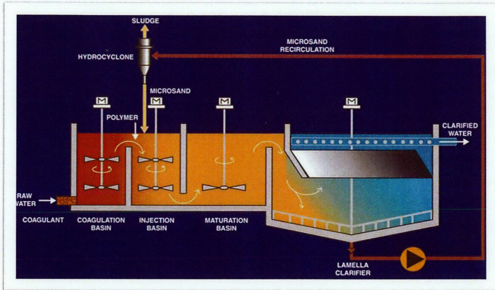
Figure 6-2. ACTIFLO® Process
